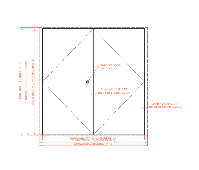
8000 – EI60 Series – 1 hr fire rated – stone frame – stone type door – 3 point lock – double door – insulated 8000-EI60-1FR-SF-ST-3PL-DD
