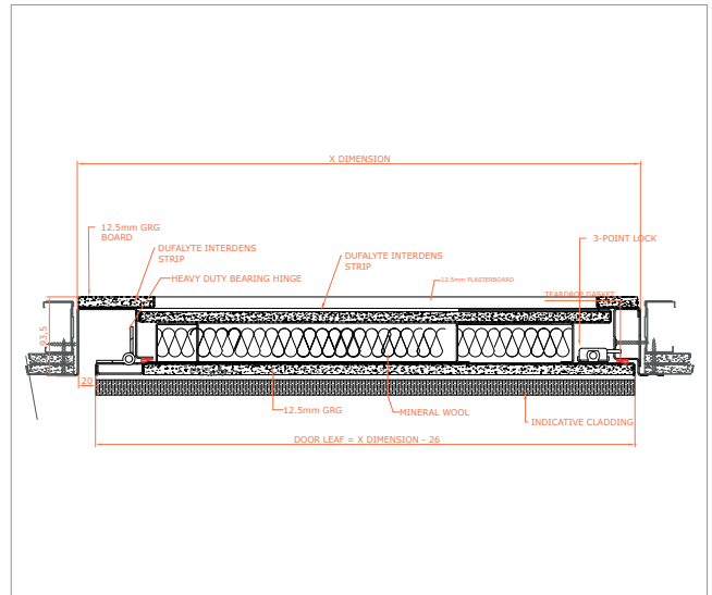
8000 - EI60 Series – 1 hr fire rated – stone frame – stone type door – 3 point lock – single door – insulated 8000-EI60-1FR-SF-ST-3PL-SD
