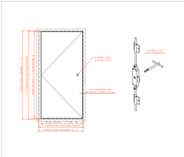
8000 - EI60 Series – 1 hr fire rated – stone frame – stone type door – 3 point lock – single door – insulated 8000-EI60-1FR-SF-ST-3PL-SD
