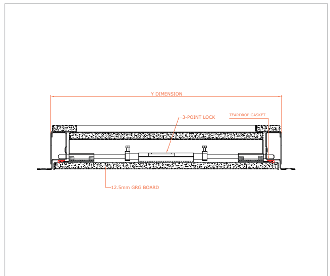
8000 – EI60 Series – 1 hr fire rated – stone frame – stone type door – 3 point lock – double door – insulated 8000-EI60-1FR-SF-ST-3PL-DD
